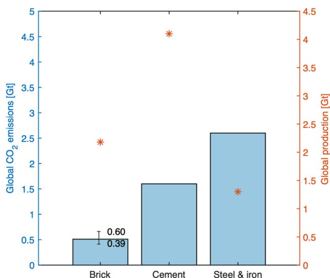
Figure 4. Estimated global production and GHG emissions from FCB, cement, and steel. The left axis shows the global GHG emissions associated with the production of brick, cement, and steel, reflected as bars. The right axis shows the global production of these materials, shown as “*”.
