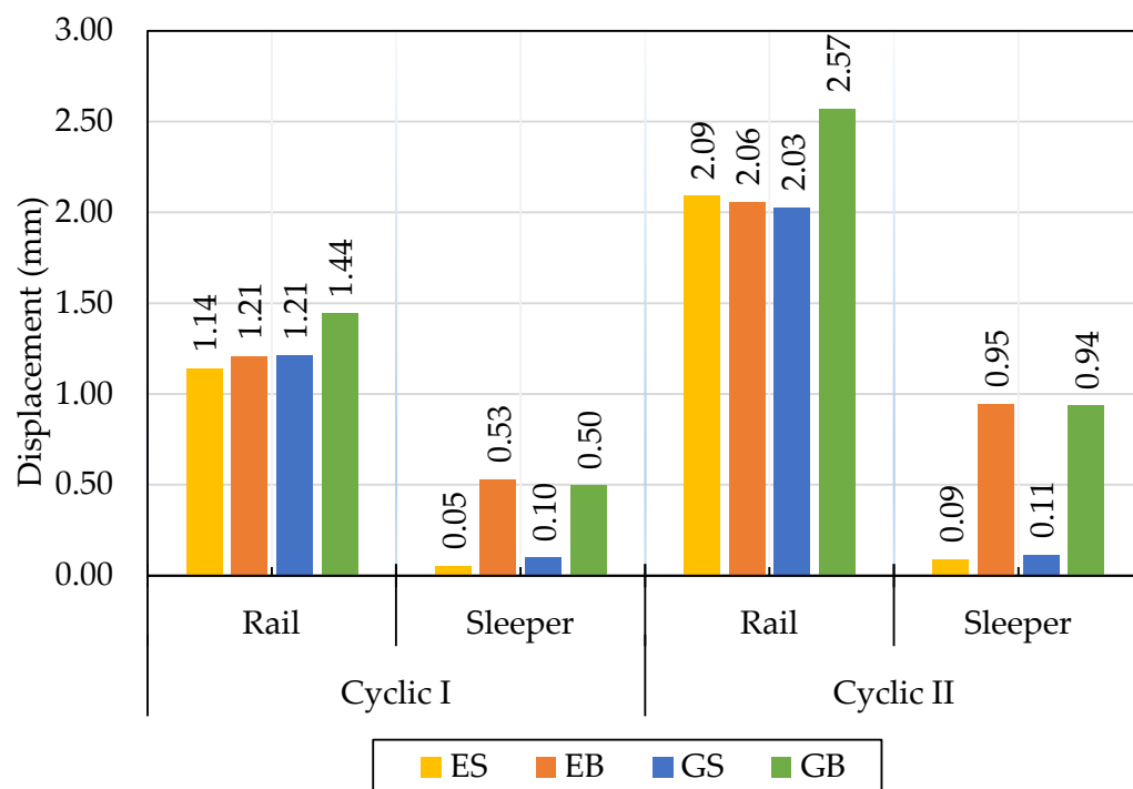
Figure 14. Average absolute displacements of the rails and sleepers under cyclic loading (slab in the slab track case), as illustrated by Esen, et al. [48].
