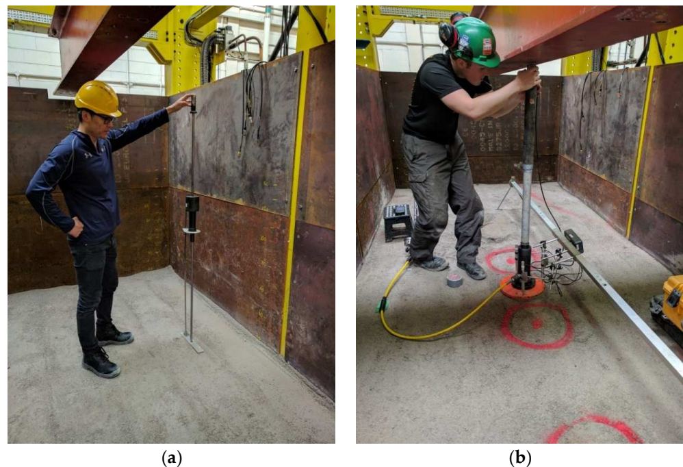
Figure 2. In situ soil parameter tests: (a) Dynamic Cone Penetrometer (DCP) and CBR investigation and (b) Plate Load Test (PLT) and E_{V2} investigation.
