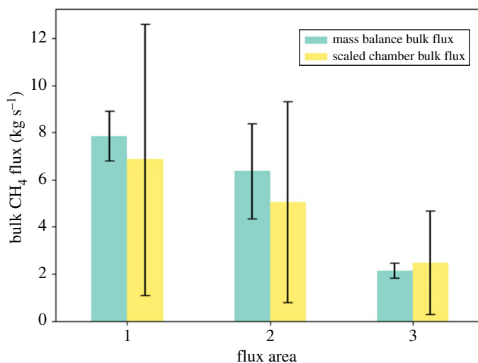
Figure 5. Bar plot comparison of bulk CH 4 flux from the three flux areas for the mass balance method and the upscaled chamber fluxes from the MAMM project. Error bars indicate the 1-σ standard deviation flux uncertainty in each case. (Online version in colour.)
