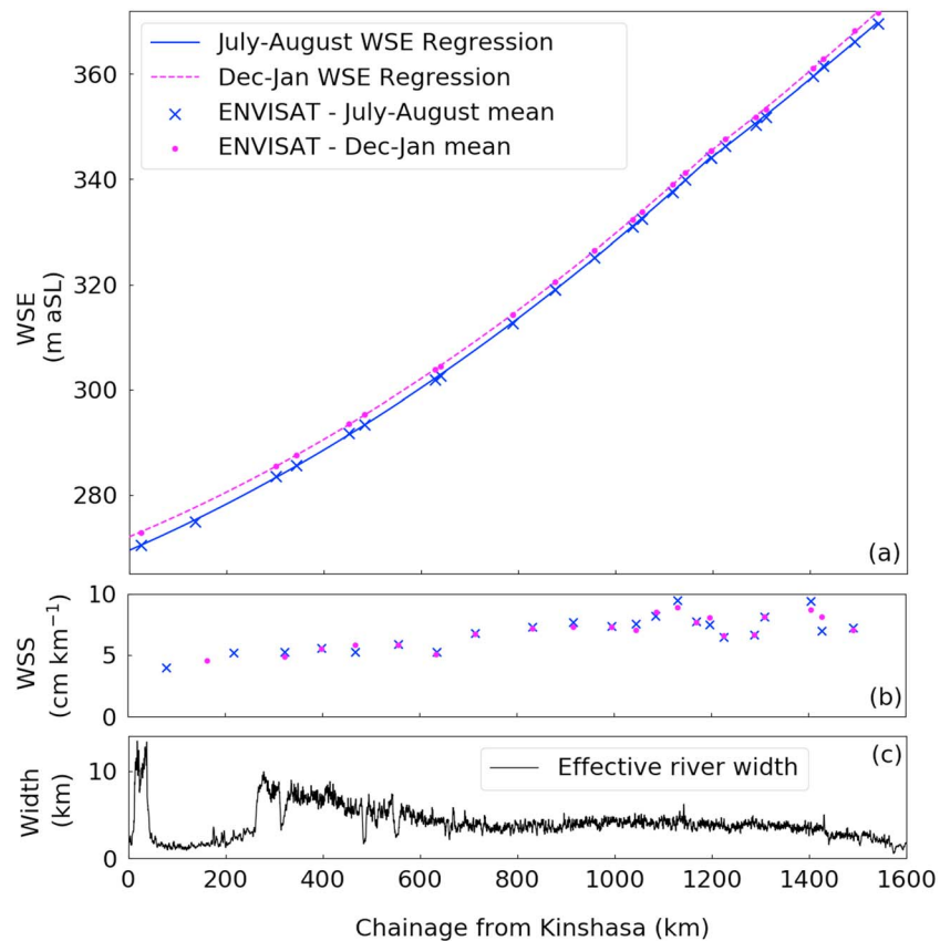
Figure 2. Longitudinal sections through the Congo middle reach main stem: (a) mean ENVISAT water surface elevations (WSEs) for July–August (low flow) and December–January (high flow), each with second-order polynomial curves fitted between chainage 0–1,200 km and 1,200–1,600 km; (b) low and high water surface slopes (WSS) calculated for each pair of mean WSEs; (c) effective river width derived from Landsat Imagery (O’Loughlin et al., 2013).
