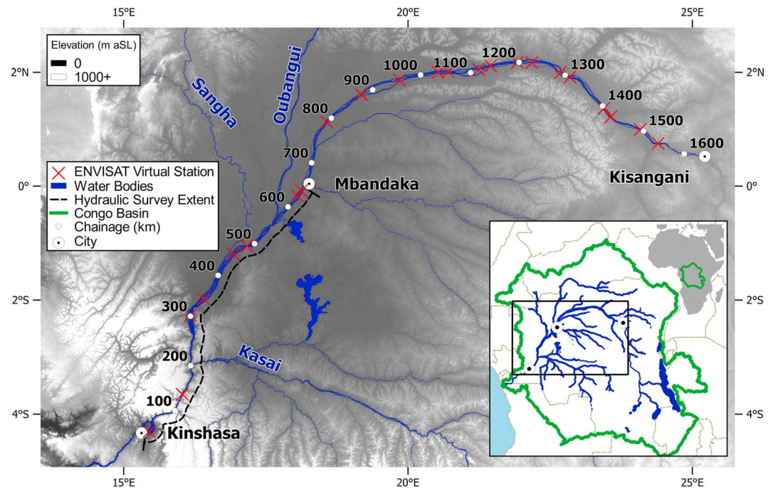
Figure 1. Map showing hydraulic survey extent and main stem ENVISAT Virtual Station locations (Santos da Silva et al., 2010). “Chainage” is river distance measured upstream of Kinshasa. Malebo Pool is situated at chainage 0–50 km, The Chenal runs from chainage 50–270 km. Three lateral constrictions in river width are located at chainage 300, 480, and 550 km. Elevations are from MERIT (Yamazaki et al., 2017); water bodies are from LANDSAT (CARPE, 2017; O’Loughlin et al., 2013).
