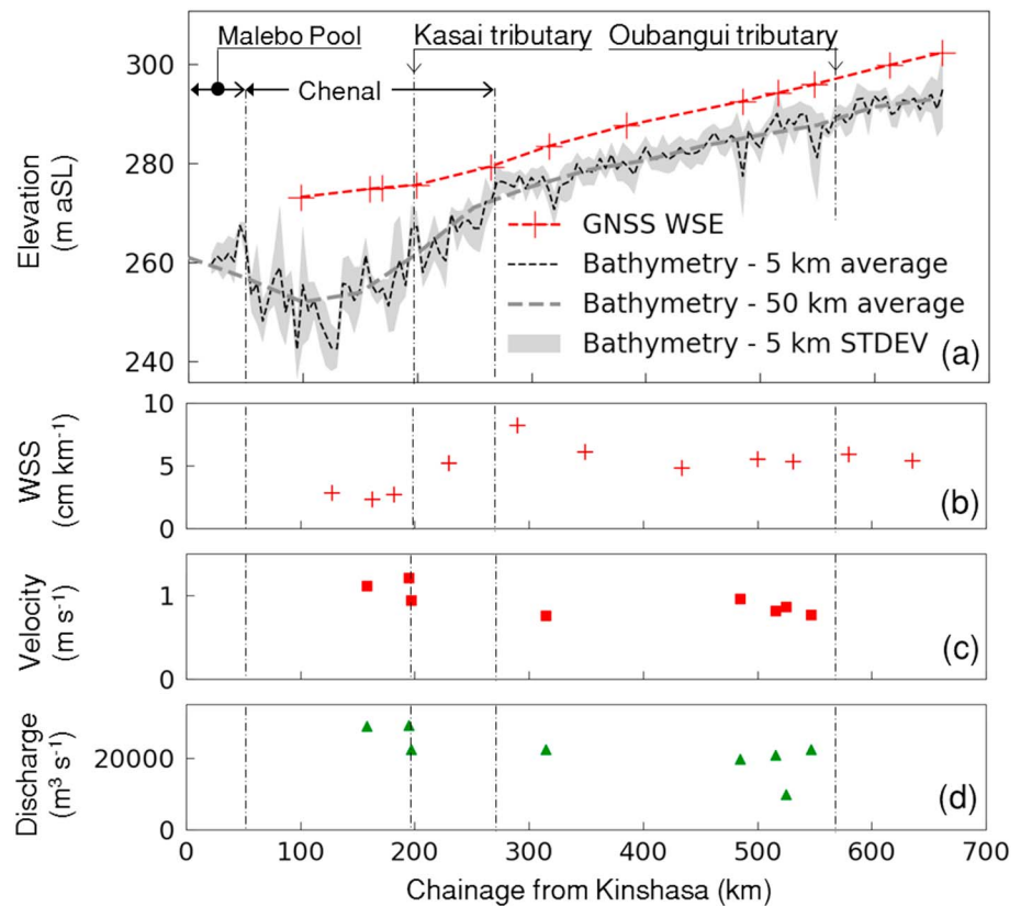
Figure 3. Key field campaign results plotted longitudinally: (a) water surface elevations (WSEs) measured with Global Navigation Satellite System (GNSS), Longitudinal Bathymetry measured with sonar and averaged over 5- and 50-km intervals; (b) water surface slope (WSS) calculated from each WSE pair; (c) acoustic Doppler current profiler measured cross-sectional average velocities; (d) acoustic Doppler current profiler measured discharge (including individual channel thread measurement at chainage 525 km). STDEV = Standard deviation.
