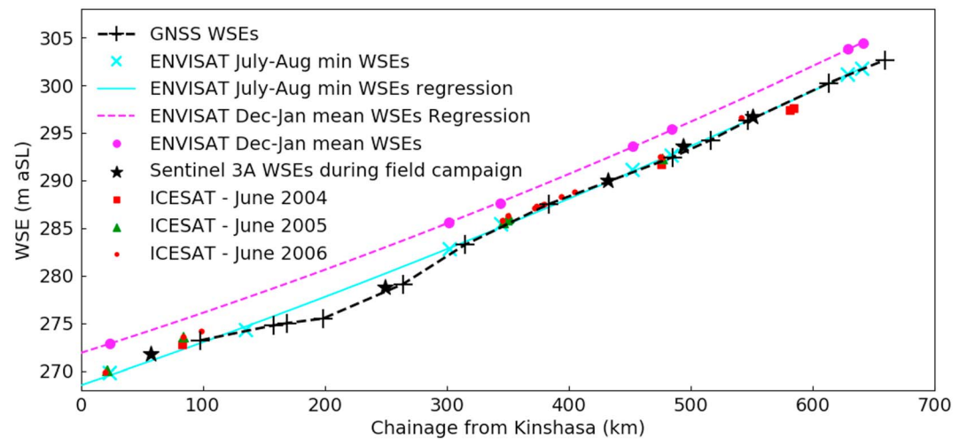
Figure 4. Plot of Global Navigation Satellite System (GNSS) water surface elevations (WSEs) and comparative low-flow altimetry WSEs from ENVISAT, Sentinel-3A, and ICESAT. High-flow (mean December and January) ENVISAT WSEs are also shown to convey the magnitude of flood-wave amplitude. GNSS WSEs are linearly interpolated piecewise. Sentinel 3A WSEs are linearly interpolated temporally to derive WSEs during field campaign.
