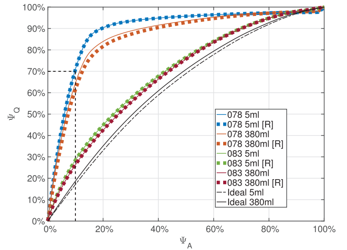
Fig. 6. Comparing area versus mass flow of blood for each device at the mid plane cross-section ( l/2 ). Coloured solid lines represent forward flow, coloured dotted lines represent the [R]reverse flow. For the idealised geometry the two mass flow rates ( 5 \text{ mL min}^{-1} and 380 \text{ mL min}^{-1} ) are plotted in black with no reverse flow, since the geometry is symmetrical. (For interpretation of the references to colour in this figure legend, the reader is referred to the web version of this article.)
