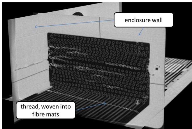
Fig. 2. Sliced 3D model reconstructed from \mu\text{CT} 2D images including a thread woven into to maintain a minimum distance between the fibres.
